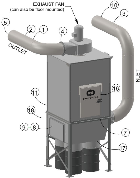
TYPICAL DUST COLLECTOR (For illustration only)
