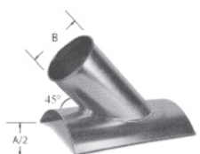
Cut In
