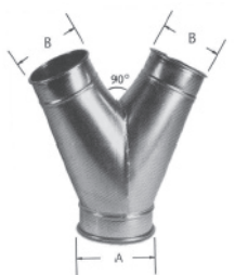
Y-Branch Fitting
