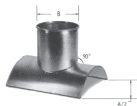
Tap In
