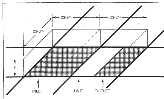
Model DC5
